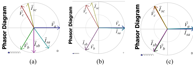
Fig. 10. Simulated phasor diagrams of v_{sx} and i_{sx} for mixed inductive and capacitive loads compensation: (a) before compensation, (b) after TCLC-HAPF (by the conventional method [18]) compensation, and (c) after TCLC-HAPF (by the proposed design method) compensation.
