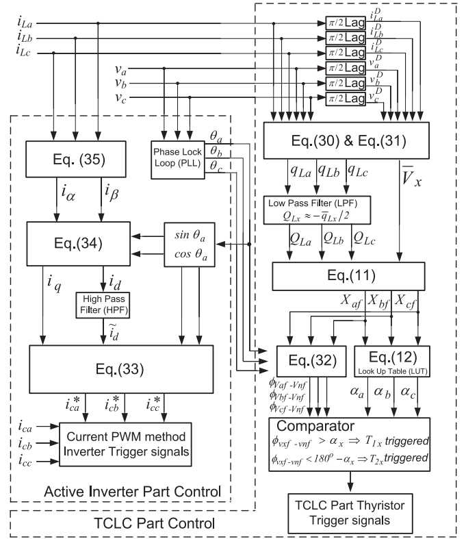
Fig. 4. Control block diagram of TCLC-HAPF.
