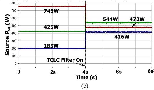
Fig. 7. Dynamic performance by using TCLC-HAPF with the conventional design method [18] for mixed inductive and capacitive loads compensation: (a) v_{sx} and i_{sx} , (b) Q_{sx} , and (c) P_{sx} .
