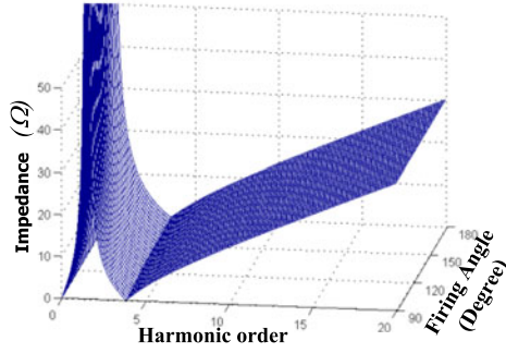
Fig. 3. Absolute value of X_{xn} and active impedance X_{ACTxn} under different harmonic orders.
