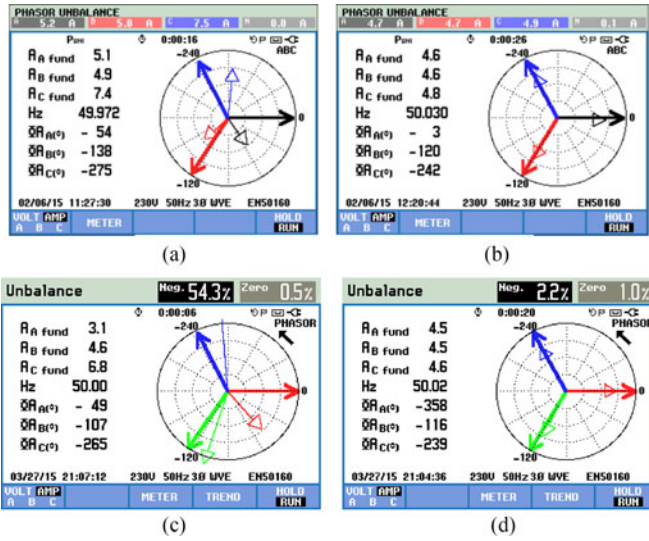
Fig. 14. Experimental phasor diagrams of v_{sx} and i_{sx} compensation: (a) before compensation for unbalanced inductive loads, (b) after TCLC-HAPF compensation for unbalanced inductive loads, (c) before compensation for mixed inductive and capacitive loads, and (d) after TCLC-HAPF compensation for mixed inductive and capacitive loads.
