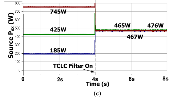
Fig. 8. Dynamic performance by using TCLC-HAPF with the proposed design method for mixed inductive and capacitive loads compensation: (a) v_{sx} and i_{sx} , (b) Q_{sx} , and (c) P_{sx} .
