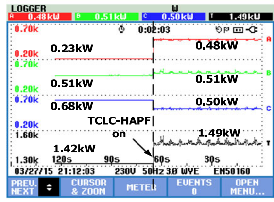
Fig. 13. Dynamic mixed inductive and capacitive loads compensation by using TCLC-HAPF with the proposed design: (a) v_{sx} and i_{sx} , (b) Q_{sx} , and (c) P_{sx} .
