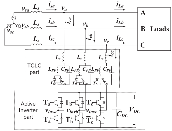
Fig. 1. Circuit configurations of the TCLC-HAPF.
