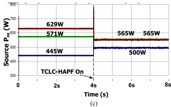
Fig. 5. Dynamic performance by using TCLC-HAPF with conventional design method [18] for unbalanced inductive loads compensation: (a) v_{sx} and i_{sx} , (b) Q_{sx} , and (c) P_{sx} .
