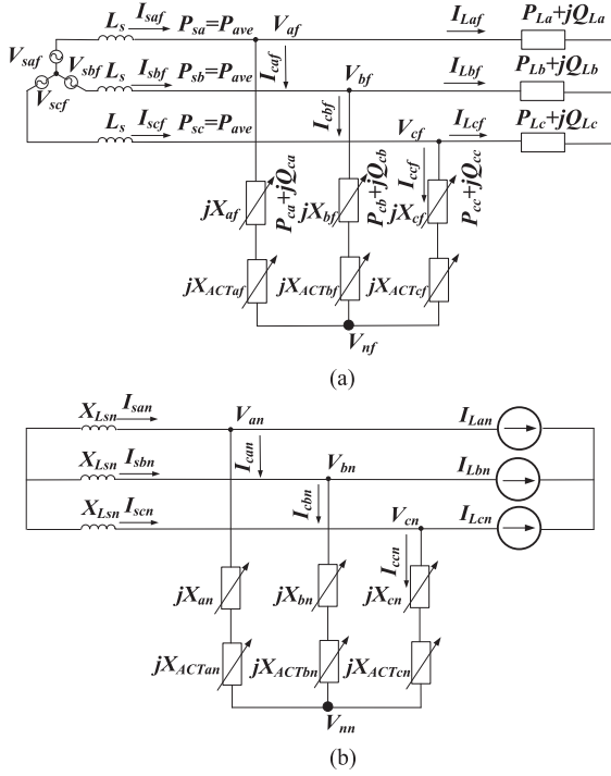
Fig. 2. Three-phase TCLC-HAPF modeling for unbalanced compensation: (a) at fundamental frequency and (b) at harmonic frequency.
