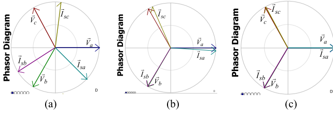
Fig. 9. Simulated phasor diagrams of v_{sx} and i_{sx} for unbalanced inductive loads compensation: (a) before compensation, (b) after TCLC-HAPF (by the conventional method [18]) compensation, and (c) after TCLC-HAPF (by the proposed design method) compensation.
