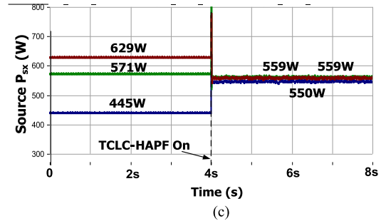
Fig. 6. Dynamic performance by using TCLC-HAPF with the proposed design method for unbalanced inductive loads compensation: (a) v_{sx} and i_{sx} , (b) Q_{sx} , and (c) P_{sx} .
